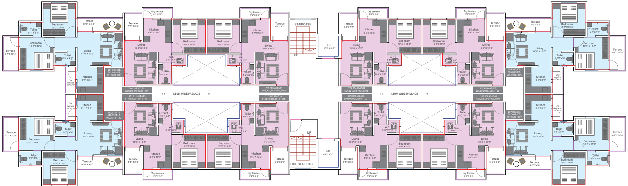
Typical Floor Plan
